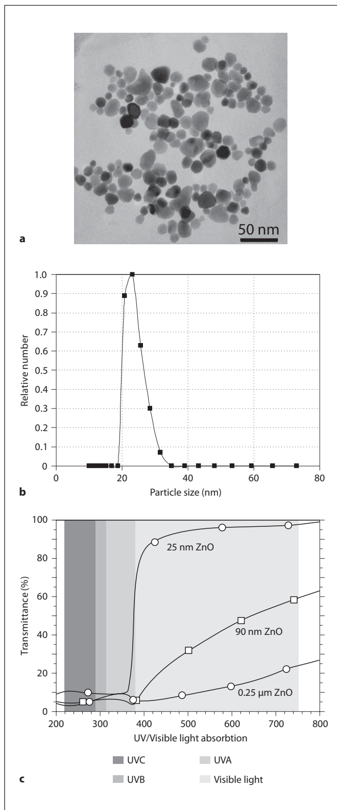
Fig. 1. a TEM picture of coated ZnO particles. b PCS size distribution of micronized ZnO particles. c Spectral transmittance of ZnO particles in aqueous solution.
