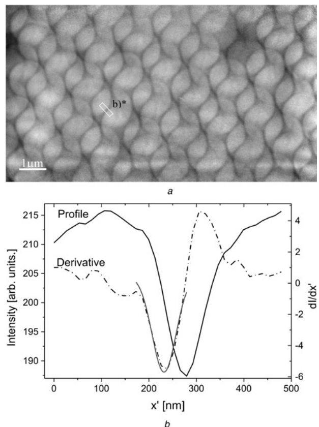
Fig. 4 Imaging with the hard X-ray microscope
