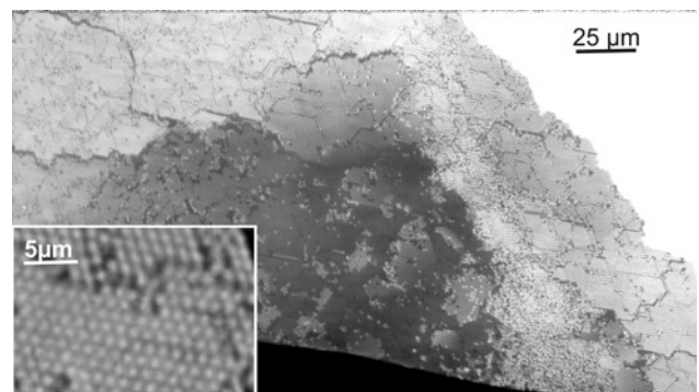
Fig. 3 In-line phase contrast image of a photonic crystal
